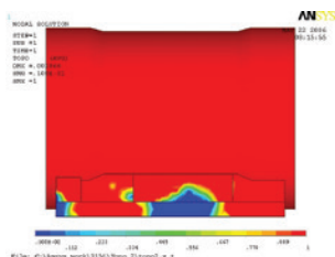
Figure 2 - Solid feet.
